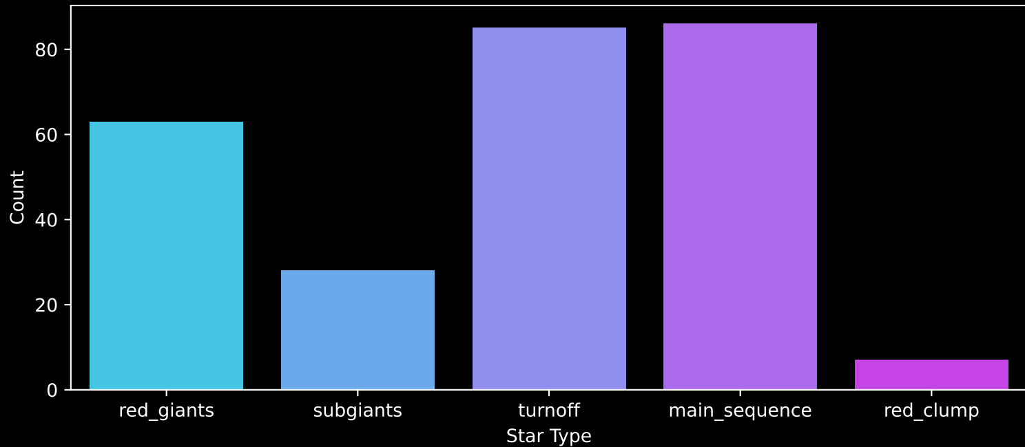
GALAH DR4 Field: [3441] Count plot of Star Type
