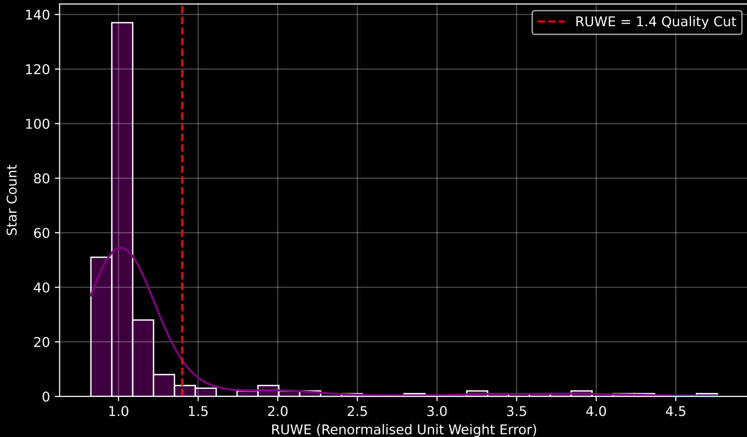
GALAH DR4 Field [3441] RUWE Distribution (n= 253)
