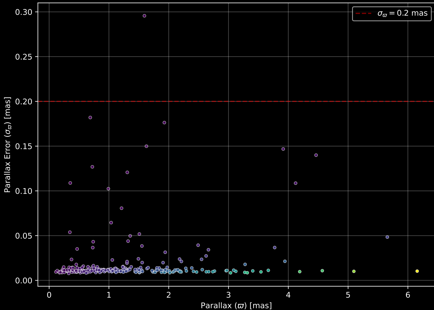
GALAH DR4 Field: [3441] Parallax Quality (n= 269)
