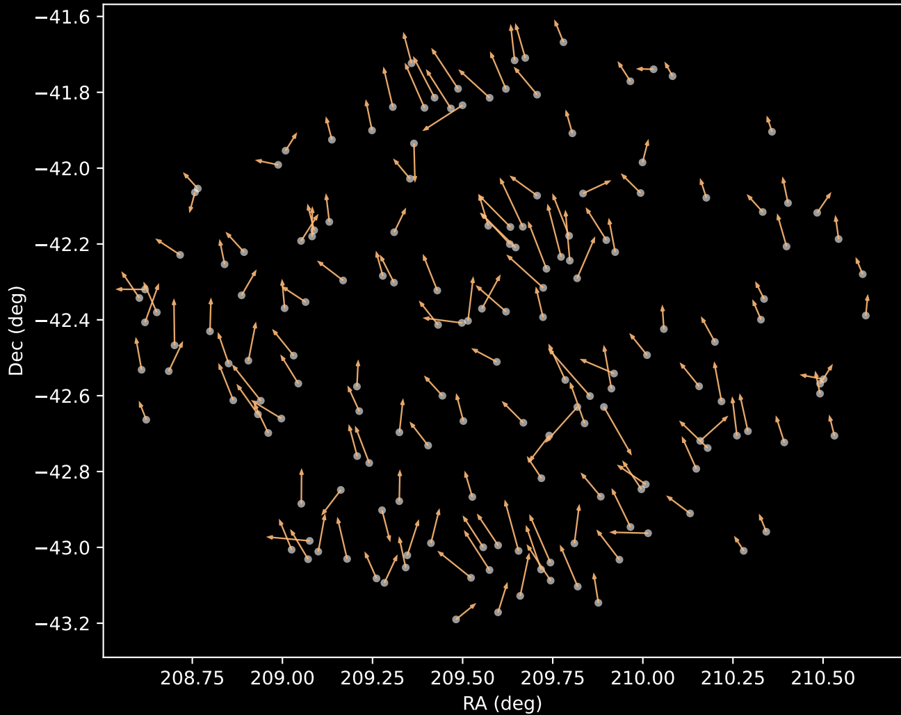
GALAH DR4 Cluster 3 Proper Motion Vectors (n=164)
