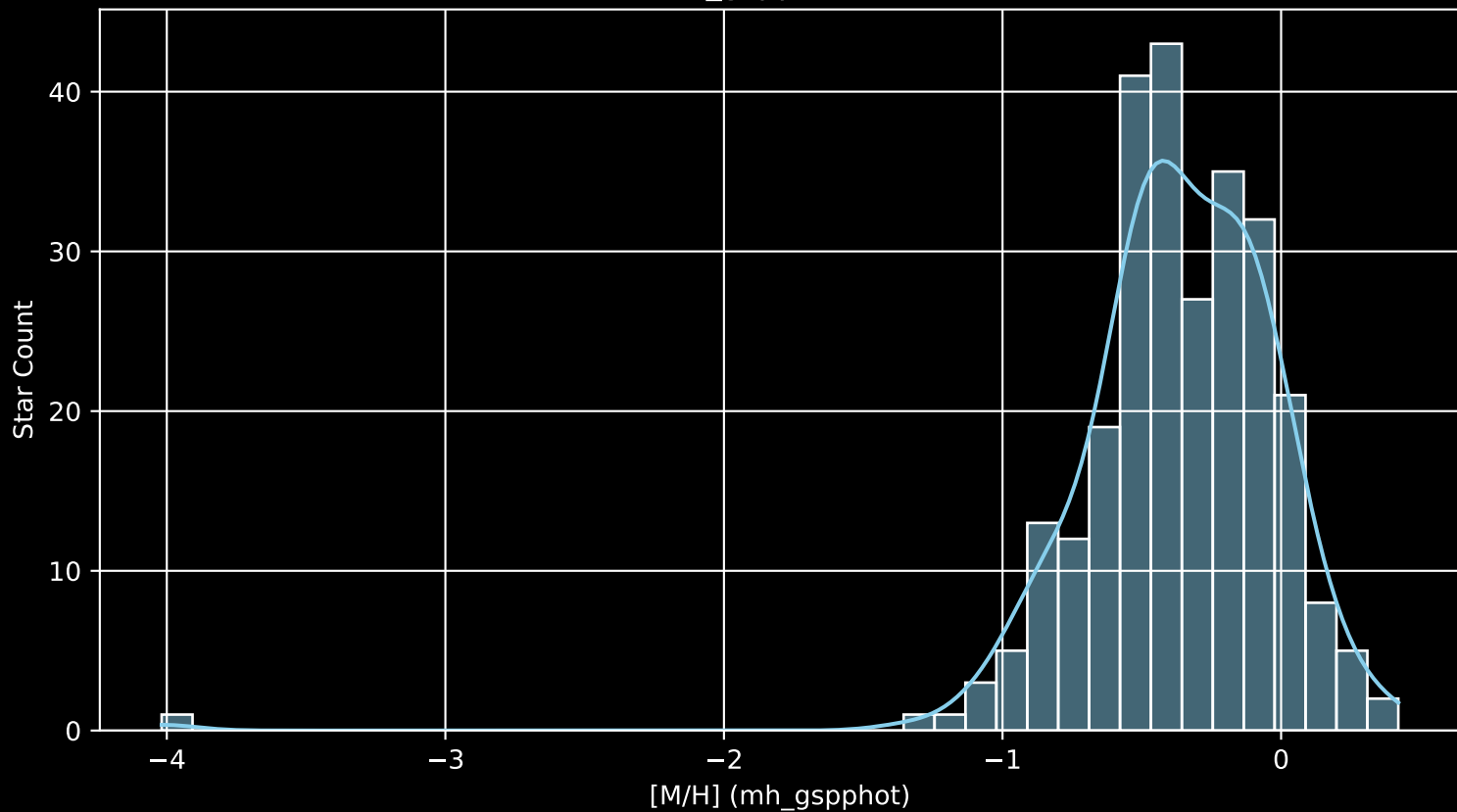
GALAH DR4 Field: [3441] [M/H] (mh_gspphot) (n= 269)
