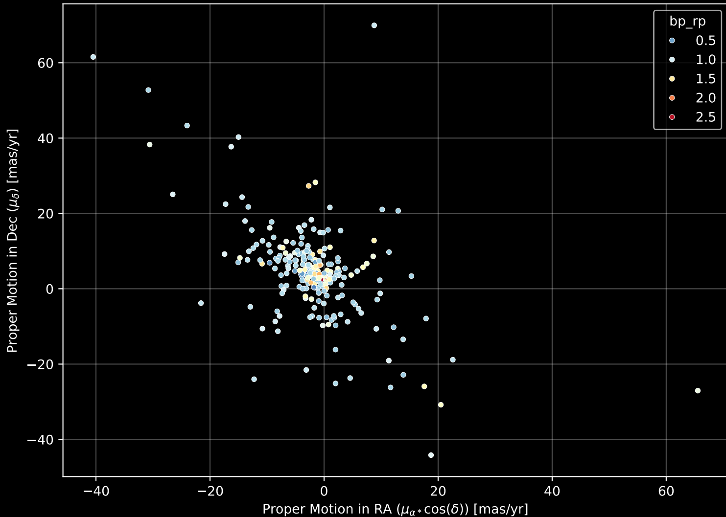
GALAH DR4 Field: [3441] Proper Motion Diagram (n= 269)
